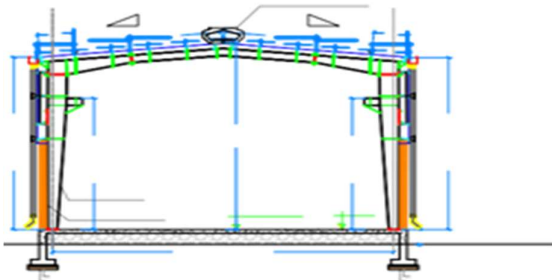
TRUSS ELEVATION DETAIL SCALE 1: 100
