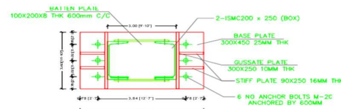
DETAILS OF BASE PLATE (BP-1)
