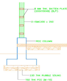
TYPICAL ELEVATION OF RCC & MS COLUMN
